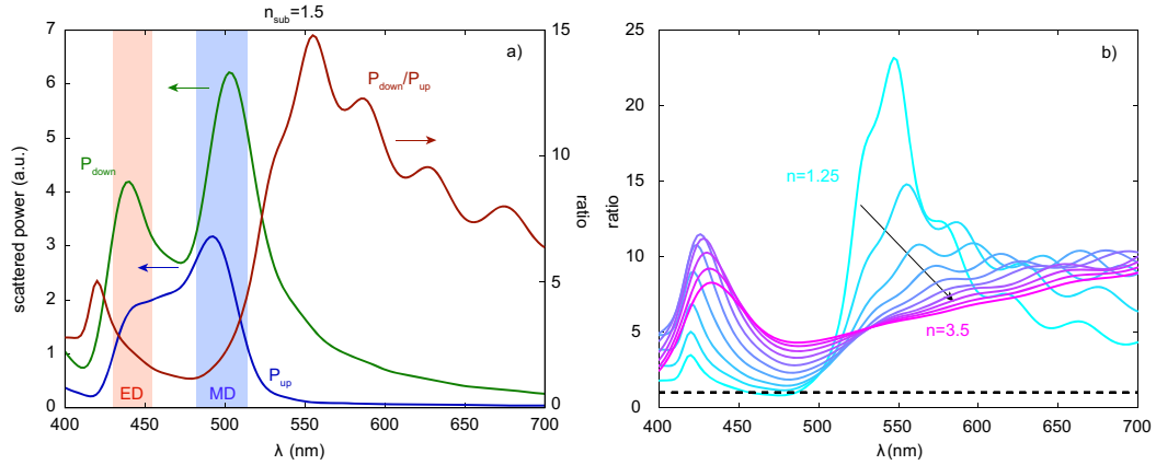
Fig. 8. (a) Back scattered power (blue), forward scattered power (green) and forward/backward ratio (red) for a d = 100 nm, h = 100 nm Si cylinder on n_{\text{sub}} = 1.5 . The red and blue shaded regions indicate the spectral range of the ED and MD resonances respectively. Note that the oscillations in the red curve for \lambda > 580 nm are due to numerical noise. (b) Forward/backward scattering ratio as a function of wavelength for different n_{\text{sub}} ranging from 1.25 to 3.5 in steps of 0.25.
