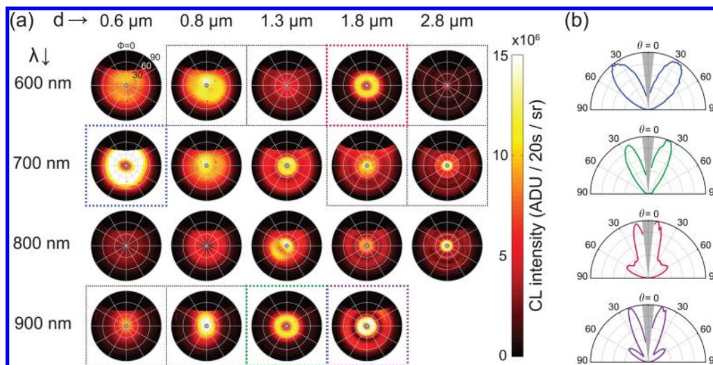
Figure 6. (a) Radiation patterns measured for different disk diameters (from left to right 0.6, 0.8, 1.3, 1.8, 2.8 \mu\text{m} ) at different detection wavelengths (from top to bottom 600, 700, 800, 900 nm) for e-beam excitation at the center of the disk. For quantitative signal strength reference, CL intensity is reported in “analog-to-digital converter units” (ADU), i.e., CCD camera counts, per steradian, and for the given 20 s acquisition time. We have no measured data for the 2.8 \mu\text{m} disk size at 900 nm. (b) 2D cross-cuts corresponding to patterns indicated by colored thick dotted boxes in (a).
