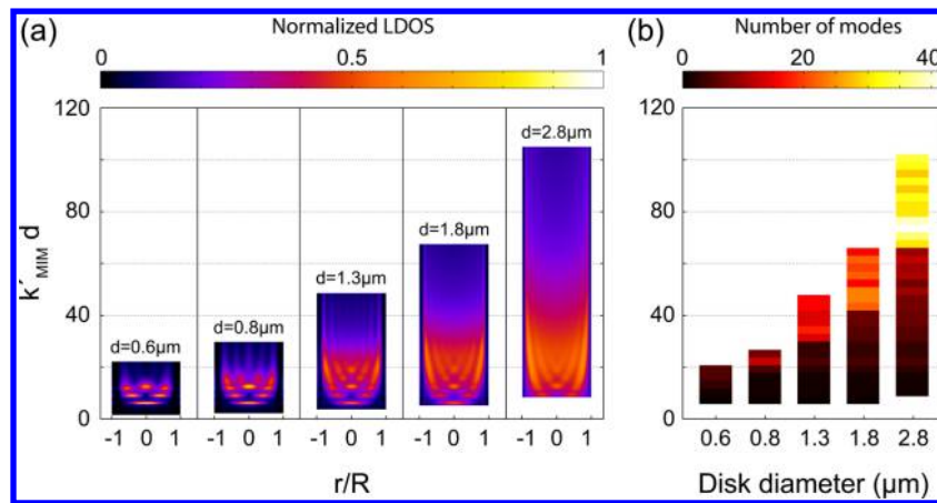
Figure 2. (a) Calculated spatial LDOS maps for five different disk sizes as a function of normalized wavenumber k'_{\text{MIM}}d and distance to the center of the disk. (b) Histogram of the number of modes participating in the calculation of (a).
