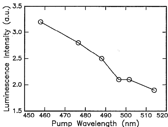
FIG. 4. Room-temperature luminescence peak intensity at \lambda=1.54\ \mu\text{m} vs pump wavelength for Er-implanted OXSEF ( 7.8 \times 10^{14} Er/cm 2 at 25 keV) after annealing for 30 min at 700 °C in vacuum.
