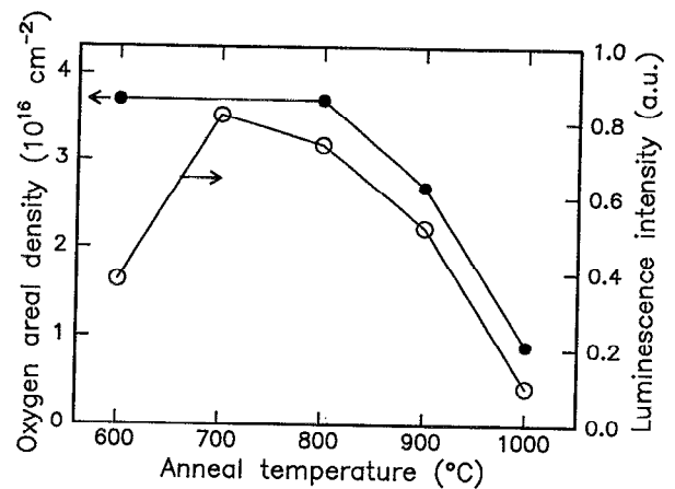
FIG. 2. Oxygen areal density (solid data points, left axis) and room-temperature luminescence intensity at 1.54 \mu\text{m} (open data points, right axis) as a function of the annealing temperature for Er-implanted OXSEF ( 7.8 \times 10^{14} Er/cm 2 at 25 keV). Annealings were performed for 30 min in vacuum.
