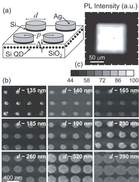
FIG. 1. (a) Array of Ag nanoparticles with diameter d and pitch p on Si-QD-doped quartz. (b) SEM images of a series of Ag nanoparticle arrays with p=400 nm and d=135 –390 nm. (c) PL intensity map over a representative Ag array ( p=400 nm, d=320 nm, and \Delta=8 nm) in 10- \mu m steps, integrated from \lambda=640 to 950 nm.
