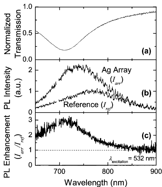
FIG. 2. Optical characterization of a representative sample ( p=400 nm, d=320 nm, and \Delta=13 nm). (a) Normalized transmission through the Ag nanoparticle array. (b) PL intensity from Si QDs in the absence (bottom curve) and presence (top curve) of Ag islands. (c) PL intensity enhancement [ratio of curves in (b)].
